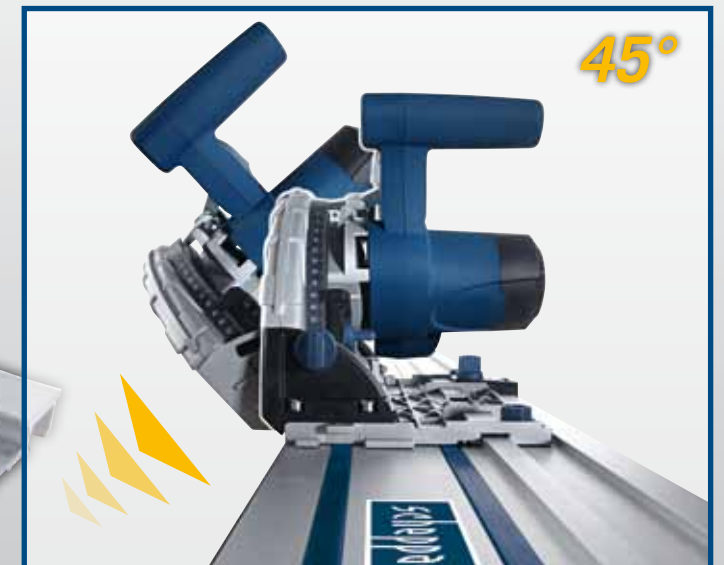
Mitre cuts with stepless angle adjustment. 0° to 45° angle adjustment
